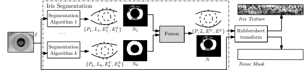
Fig. 1: Iris Segmentation Fusion Framework.
