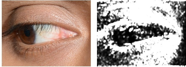
Figure 2: HoG-like features. a) original eye image; b) weighted votes for the bin starting at 120 to 140 degrees.
